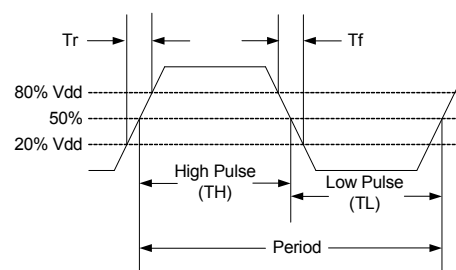
Figure 3. Output Waveform
