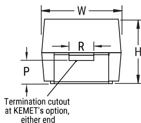
CATHODE (-) END VIEW
