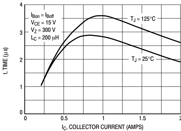
Figure 15. Inductive Storage Time, t_{st} @ h_{FE} = 5
