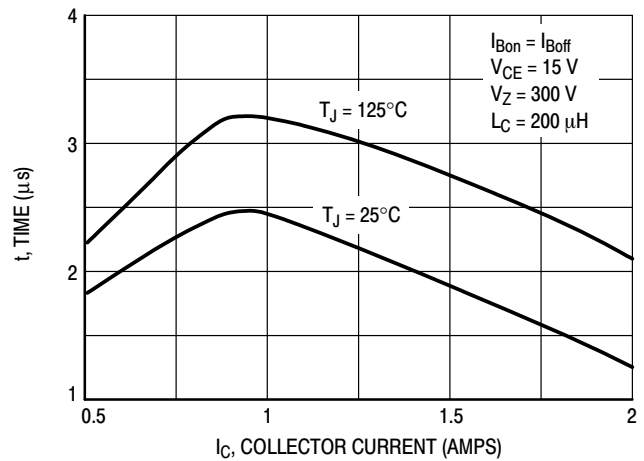
Figure 16. Inductive Storage Time, t_{st} @ h_{FE} = 10
