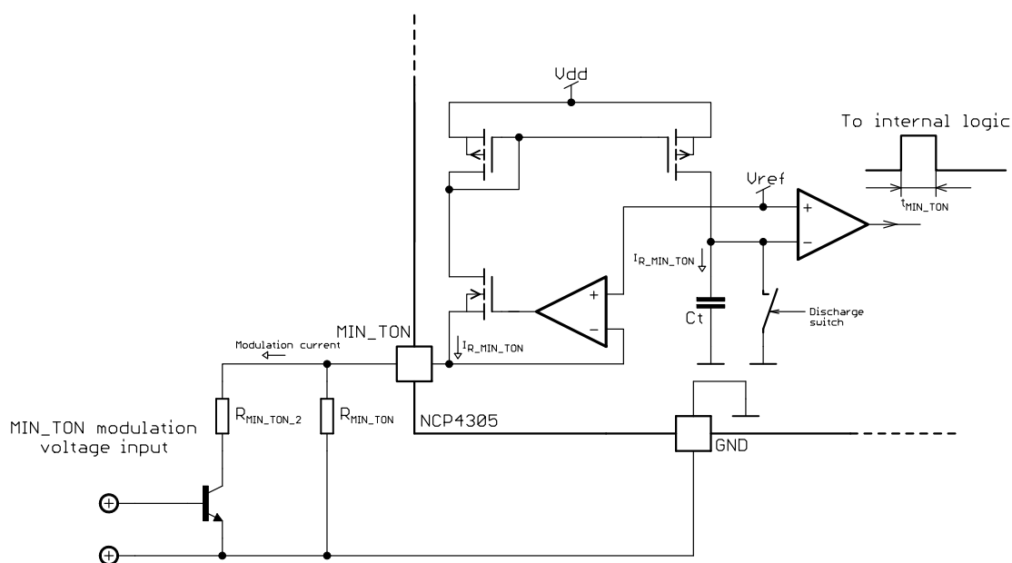
Figure 71. Possible Connection for MIN_T ON and MIN_T OFF Modulation
