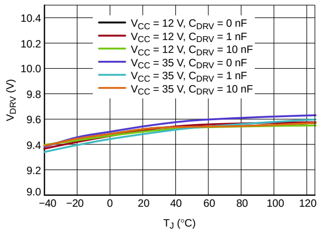
Figure 39. Driver and Output Voltage, ver. B, D and Q
