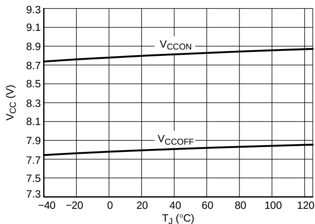
Figure 8. V_{CCON} and V_{CCOFF} Levels, ver. B, C
